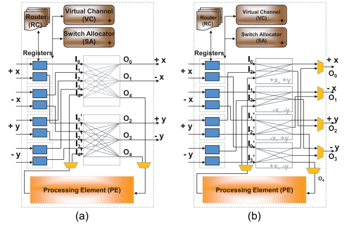
Fig. 4. (a) 2XB organization. (b) 4XB organization.
