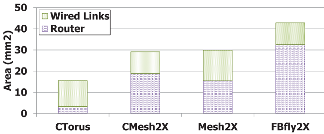
Fig. 10. Router and link area overhead of each topology.
