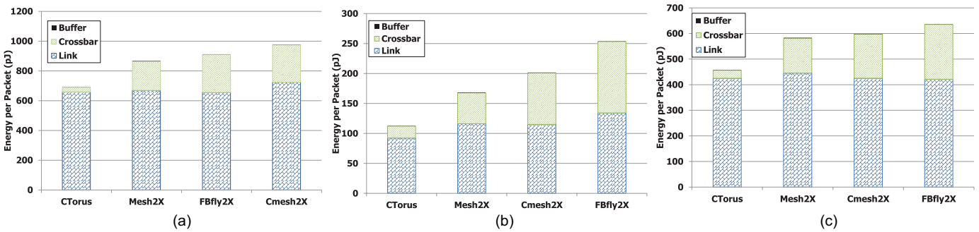
Fig. 9. Energy per packet for different traffic loads. (a) Complement. (b) Butterfly. (c) Uniform random.
