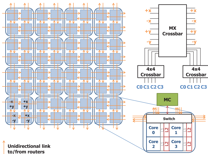
Fig. 6. CTorus topology and router design using the 4XB crossbar organization.
