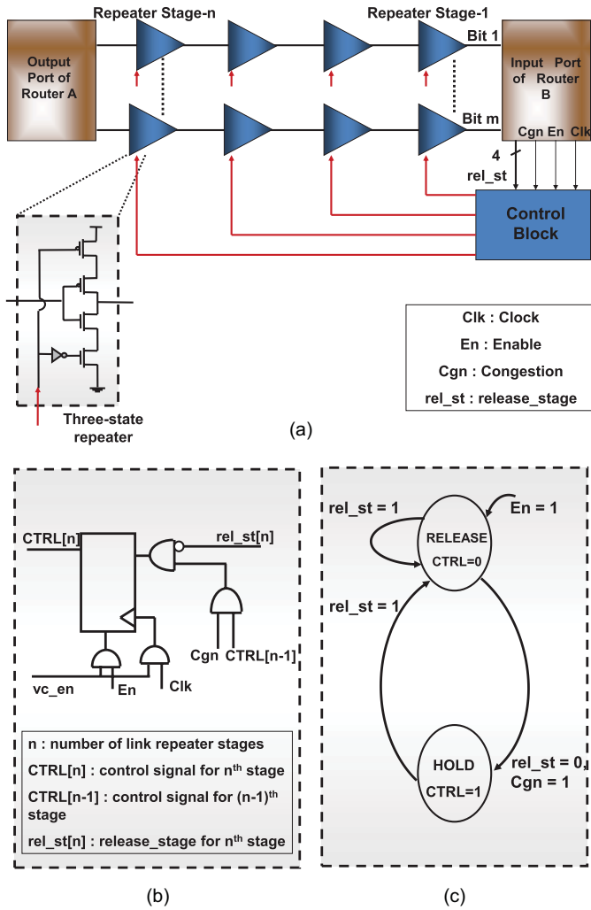
Fig. 1. (a) Link using three-state repeaters that function as channel buffers during congestion. (b) Control block implementation details. (c) State transition diagram.
