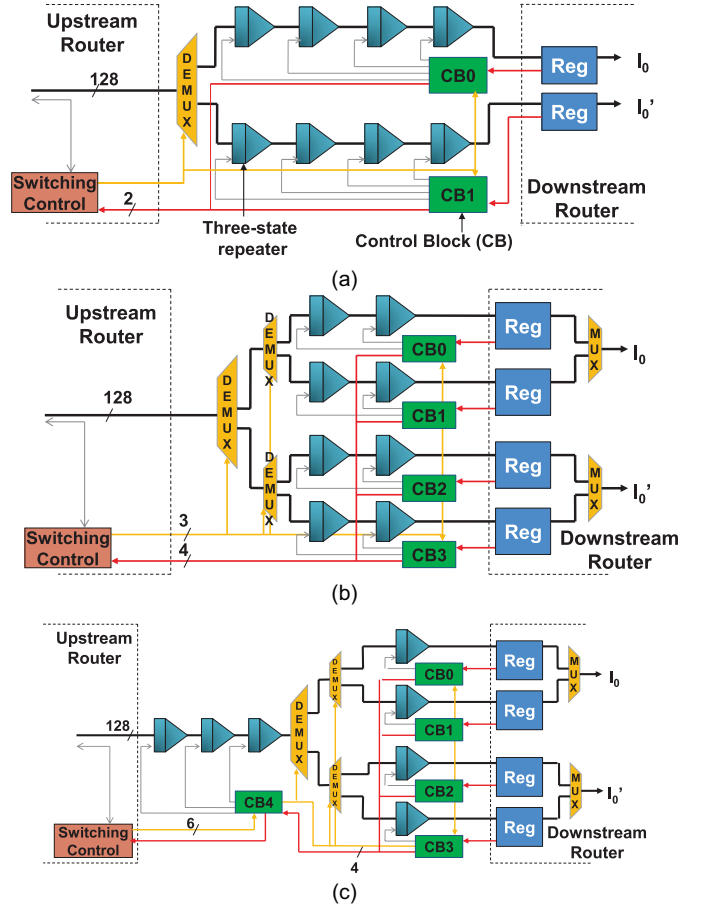
Fig. 2. (a) Four-stage (4S) channel buffer organization. (b) Two-stage (2S) channel buffer organization. (c) One-stage (1S) channel buffer organization.
