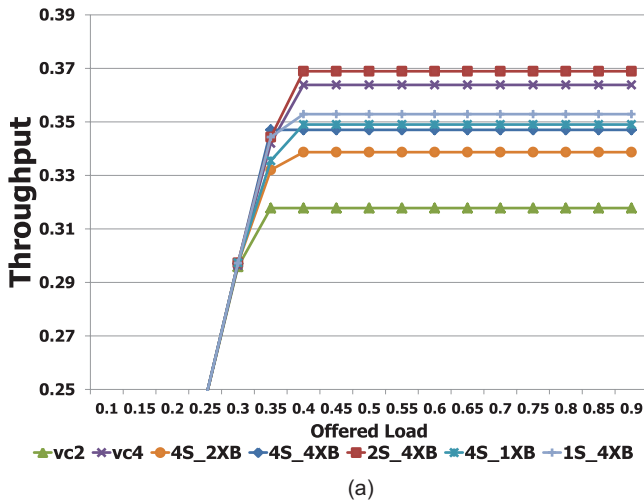
Fig. 11. Throughput and latency for different designs for uniform traffic.
