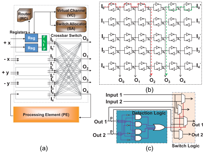
Fig. 3. (a) Dual-input single matrix crossbar (1XB) organization. (b) Example communication from dual inputs. (c) Flip logic.
