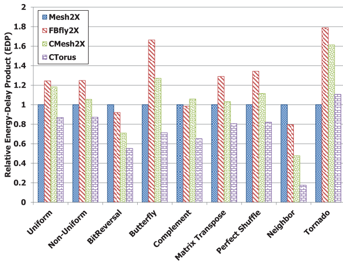
Fig. 14. Relative EDP of 64 core topologies for all synthetic traffic.
