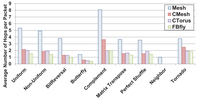
Fig. 7. Average hop count per packet for different synthetic traffic loads.
