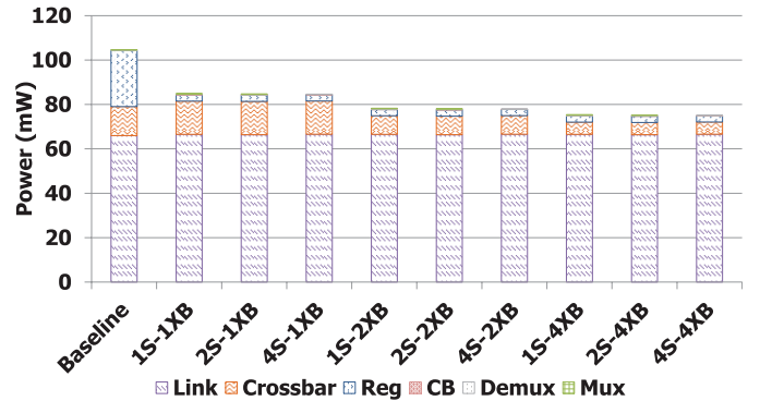
Fig. 8. Dynamic power breakdown for different design choices.
