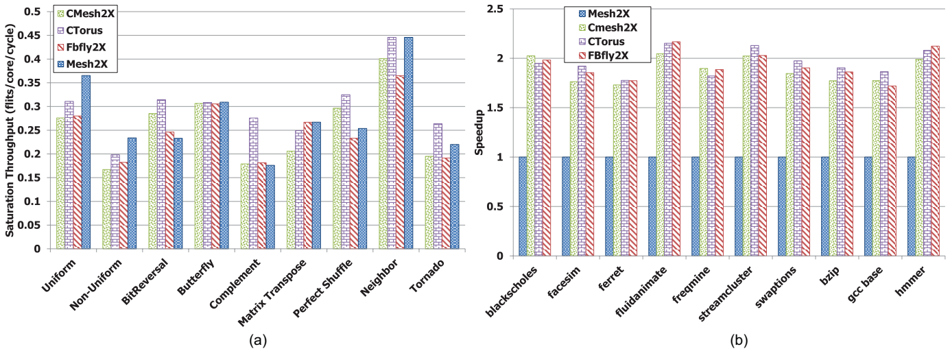
Fig. 13. (a) Saturation throughput of 64 cores for synthetic traffic patterns. (b) Speedup of 64 core topologies for SPEC2006 and PARSEC benchmarks.
