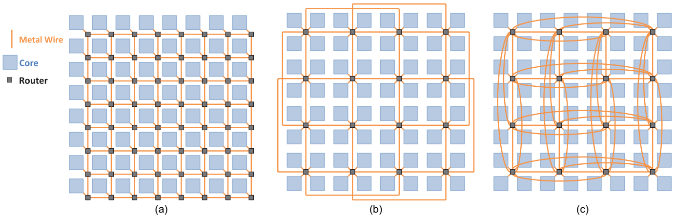
Fig. 5. (a) Mesh. (b) CMesh. (c) FBfly topologies.
