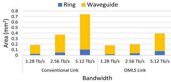
Fig. 4. Area consumption of different bandwidths.
