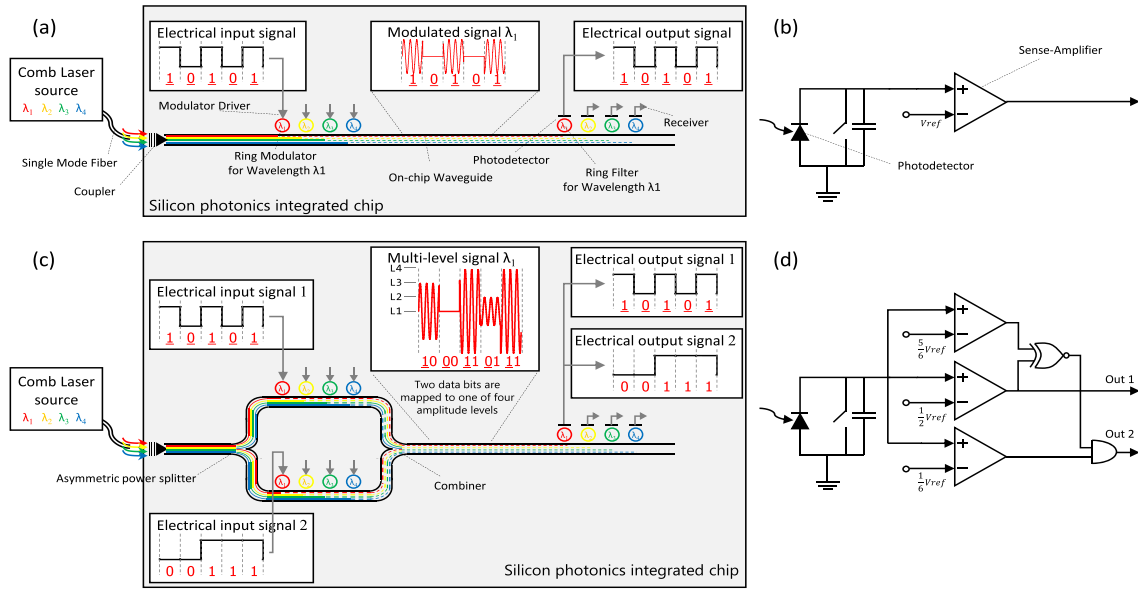
Fig. 1. (a) The conventional photonic link. (b) The current-integrating receiver. (c) The Optical Multi-Level Signaling (OMLS) link. Example of encoding a four-amplitude-level signal into a single wavelength with two input binary signals and OMLS receiver using (d) a modified current-integrating receiver.
