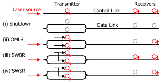
Fig. 5. Adaptive power management for the proposed OMLS link. The upper first waveguide is the control link and the lower waveguides are the data links with four operation modes respectively. The colored circle represents that the ring is tuned in and gray represents that it is tuned out.
