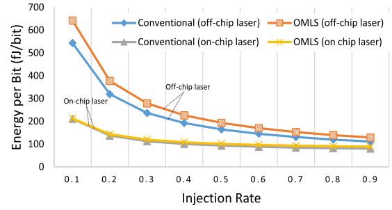
Fig. 3. Optimized energy consumption vs. injection rate of a link with 640 Gb/s bandwidth for different approaches.
