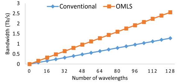
Fig. 2. The bandwidth of one singular link using both approaches.
