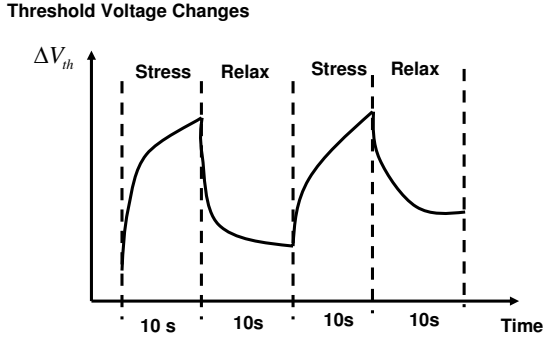
Fig. 2. NBTI PMOS Fractional Model with Both Stress and Relaxing Phases
