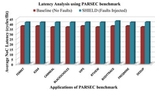
Fig. 13. 8 × 8 NoC with Shield routers using PARSEC.
