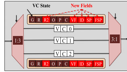
Fig. 4. Proposed input port to provide hard fault tolerance.
