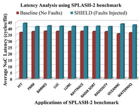
Fig. 12. 8 × 8 NoC with Shield routers using SPLASH-2.
