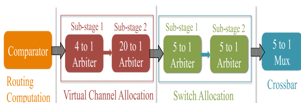
Fig. 8. Path of a flit through the router pipeline.
